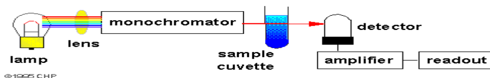
Figure 4. UV-Visible spectrophotometer
